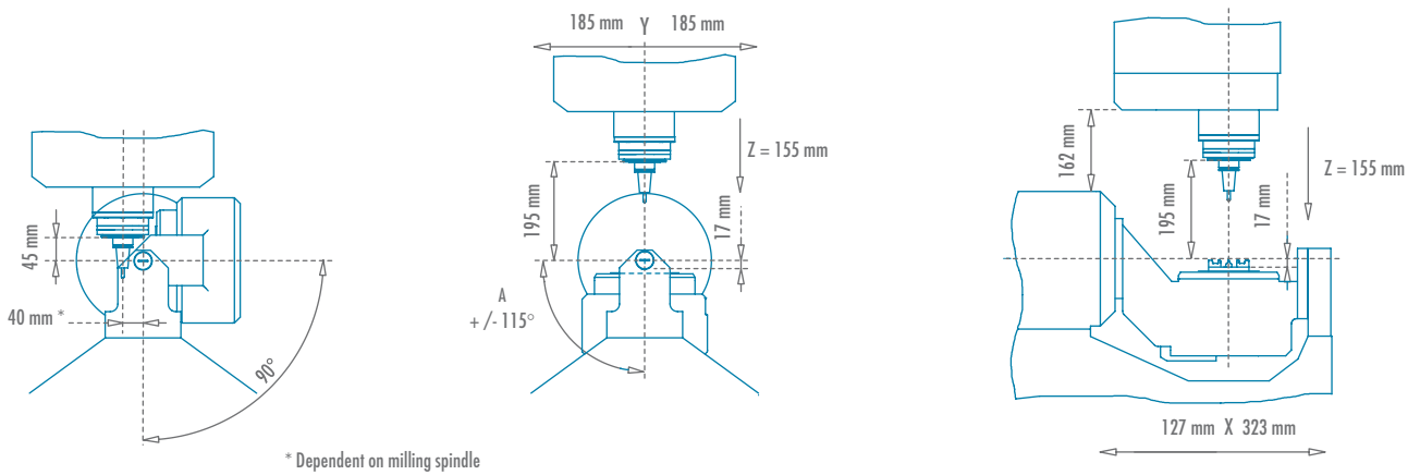
Single spindle machine with fast tool changer
